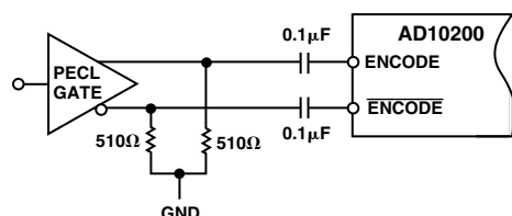
Figure 6. AC Coupling to ENCODE Inputs
