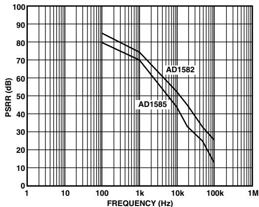
Figure 9b. Ripple Rejection vs. Frequency
