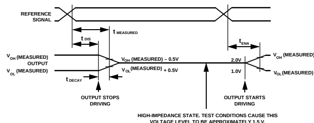
Figure 18. Output Enable/Disable
