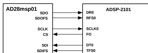
Figure 3. AD28msp01-to-ADSP-2101 Interface
