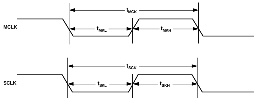
Figure 16. Clock Signals
