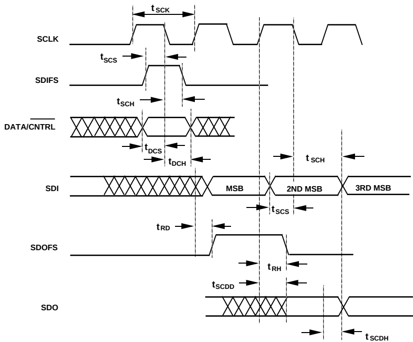
Figure 14. Serial Ports
