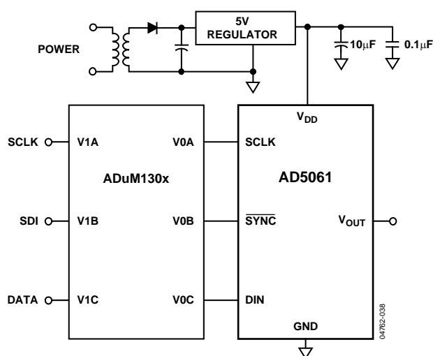
Figure 39. AD5061 with a Galvanically-Isolated Interface
