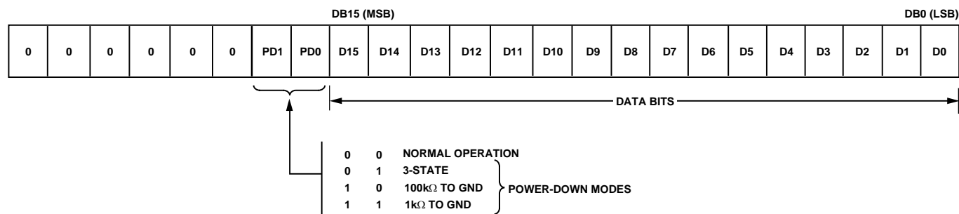
Figure 29. Input Register Contents
