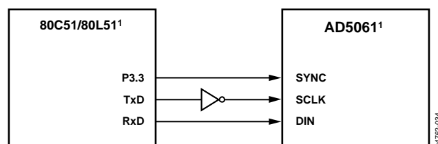
Figure 35. AD5061-to-80C51/80L51 Interface
