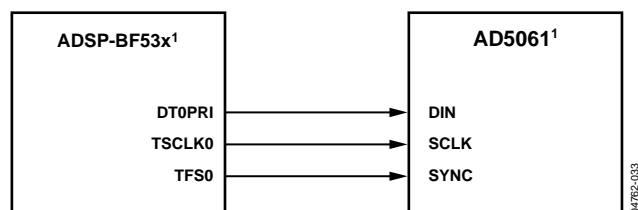
Figure 34. AD5061-to-Blackfin ADSP-BF53x Interface
