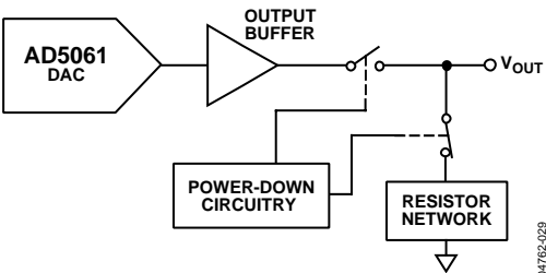
Figure 30. Output Stage During Power-Down
