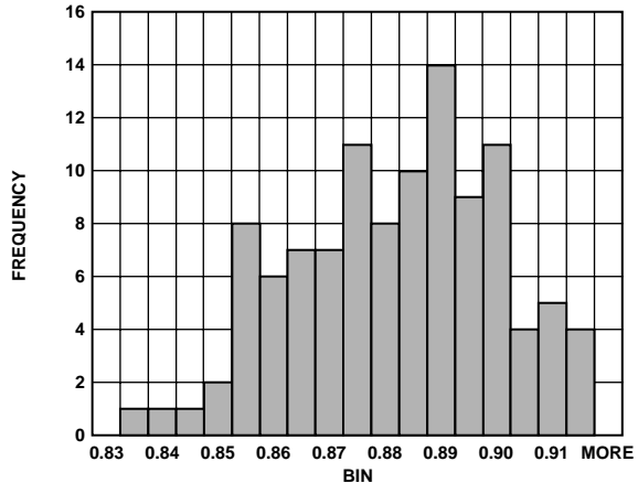
Figure 23. I_{DD} Histogram @ V_{DD} = 3\text{ V}
