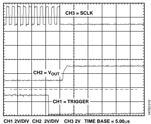
Figure 19. Exiting Power-Down
