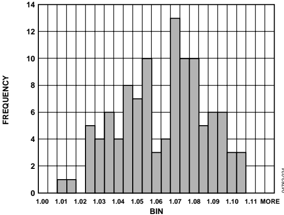
Figure 24. I_{DD} Histogram @ V_{DD} = 5\text{ V}
