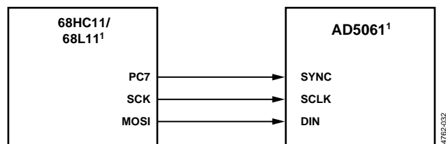
Figure 33. AD5061-to-68HC11/68L11 Interface
