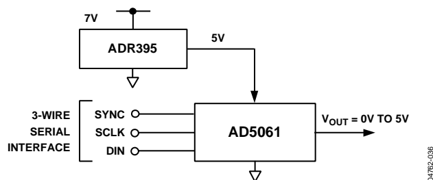
Figure 37. ADR395 as Reference to the AD5061
