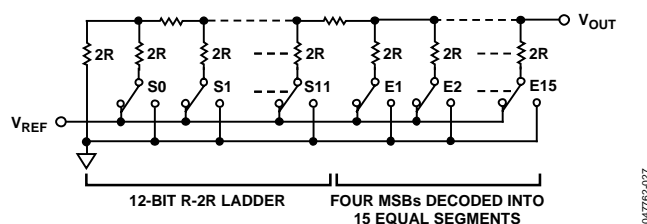
Figure 28. DAC Ladder Structure
