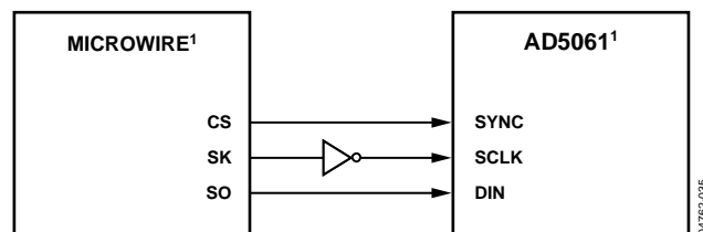
Figure 36. AD5061-to-MICROWIRE Interface
