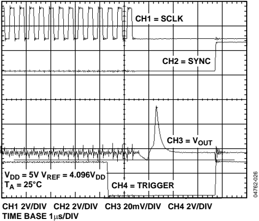
Figure 26. Exiting Software Power-Down to Glitch
