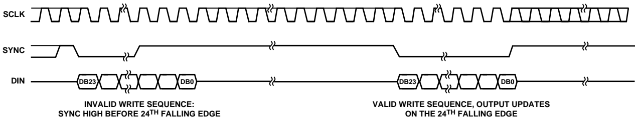
Figure 32. SYNC Interrupt Facility
