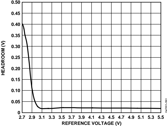
Figure 27. V_{DD} Headroom vs. Reference Voltage
