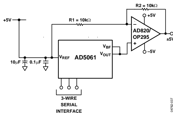
Figure 38. Bipolar Operation with the AD5061
