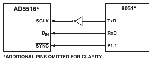
Figure 9. AD5516 to 8051 Interface
