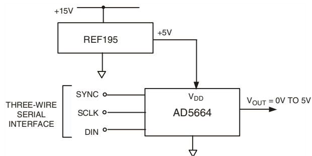
Figure 40. REF195 as Power Supply to the AD5624R/AD5644R/AD5664
