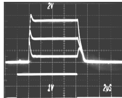
Figure 21. V_{LOG} Output for 10.7 MHz CW Input with PRUP Toggled ON and OFF; Top Trace: +5 dBm Input; Middle Trace: -35 dBm Input; Bottom Trace: -75 dBm; PRUP Input from HP8112A: 0 to 4 V, 10\ \mu\text{s} Pulsewidth with 10 kHz Repetition Rate
