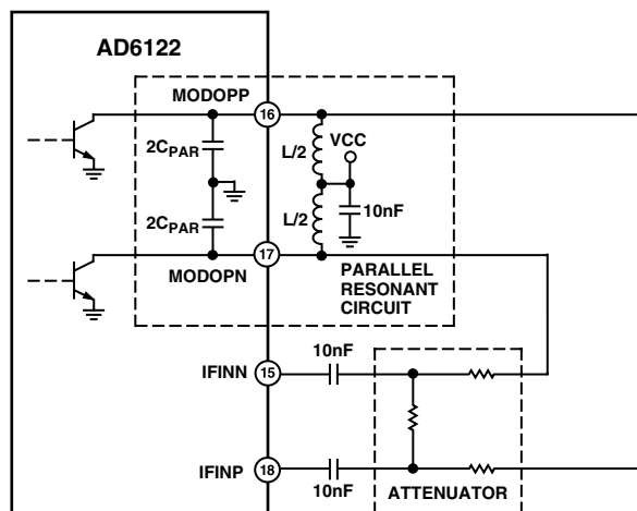
Figure 27. Roofing Filter Configuration
