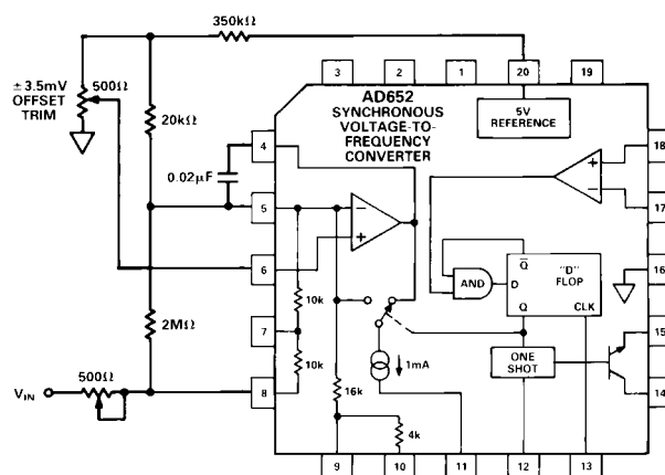
Figure 10b. PLCC Gain and Offset Trim
