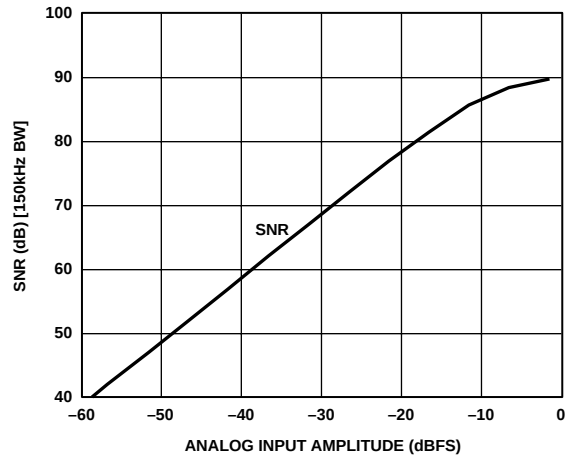
Figure 12. Noise vs. Analog Amplitude at 68 MHz
