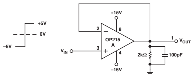
Figure 3. Slew Rate Test Circuit
