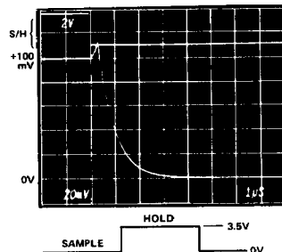
ACQUISITION TIME + 100mV to 0V
