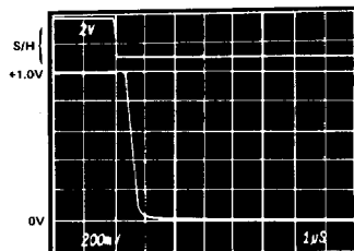
ACQUISITION TIME +1.0V to 0V
