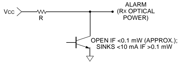
Figure 1. Receiver Electrical Schematic
