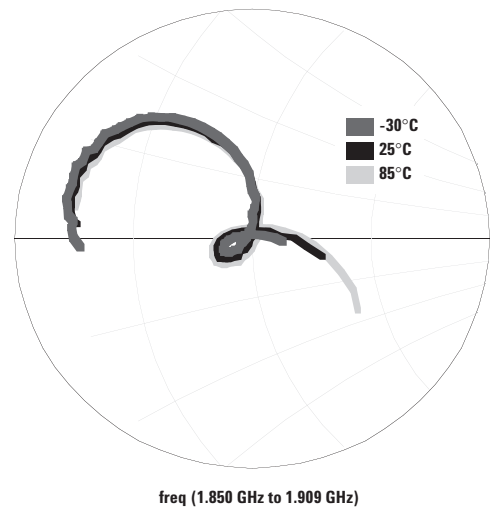
Figure 7. Tx port impedance (8 dB circle).
