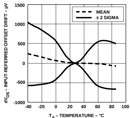
Figure 2. Input-Referred Offset Drift vs. Temperature.
