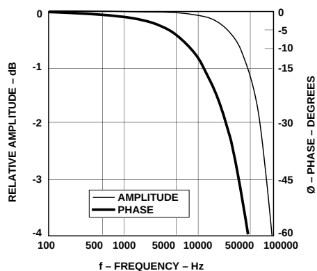
Figure 23. Typical Amplitude and Phase Response vs. Frequency.
