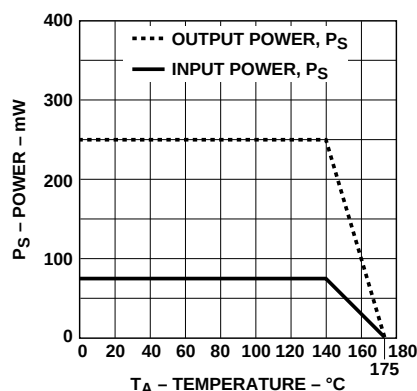
Figure 27. Dependence of Safety-Limiting Parameters on Ambient Temperature.
