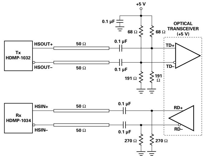
D) G-LINK INTERFACE TO OPTICAL TRANSCEIVER
