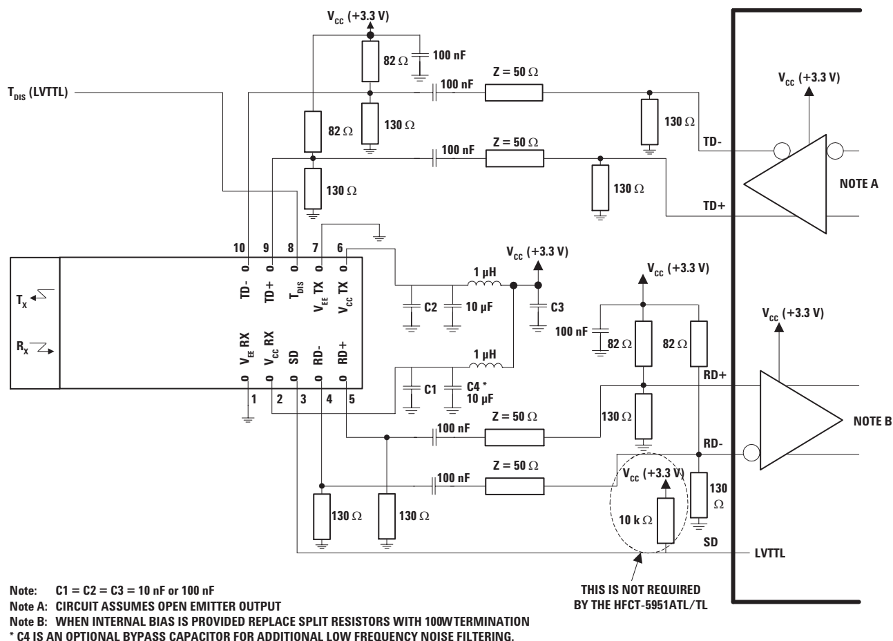
Figure 8. Recommended Interface Circuit (HFCT-5951xx)
