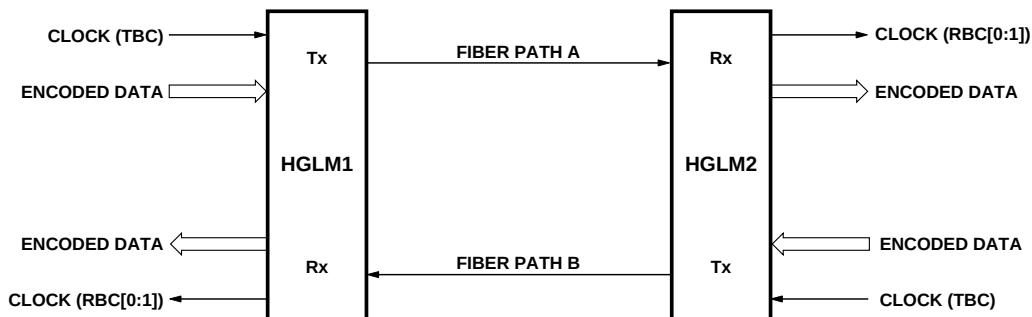
Figure 3. Full Duplex Point to Point Link.
