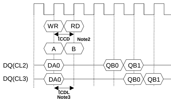
3) Write interrupted by Read (BL =2)
