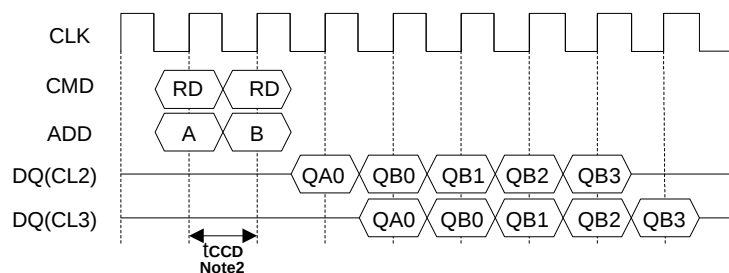
1) Read interrupted by Read (BL=4) Note 1
