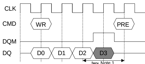
1) Normal Write (BL=4)
