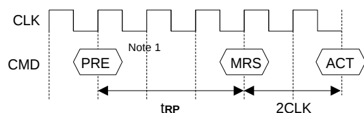
Mode Register Set
