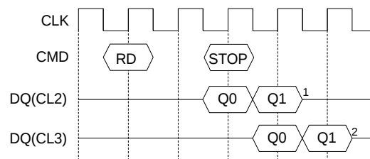
4) Read Burst Stop (BL=4)
