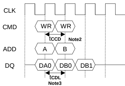
2) Write interrupted by Write (BL =2)
