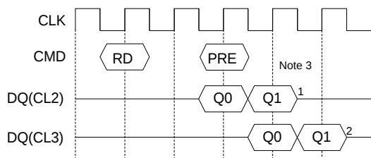
1) Read Interrupted by Precharge (BL=4)
