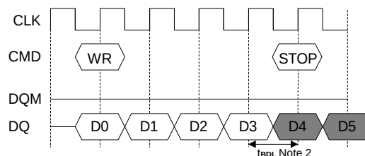
2) Write Burst Stop (BL=8)
