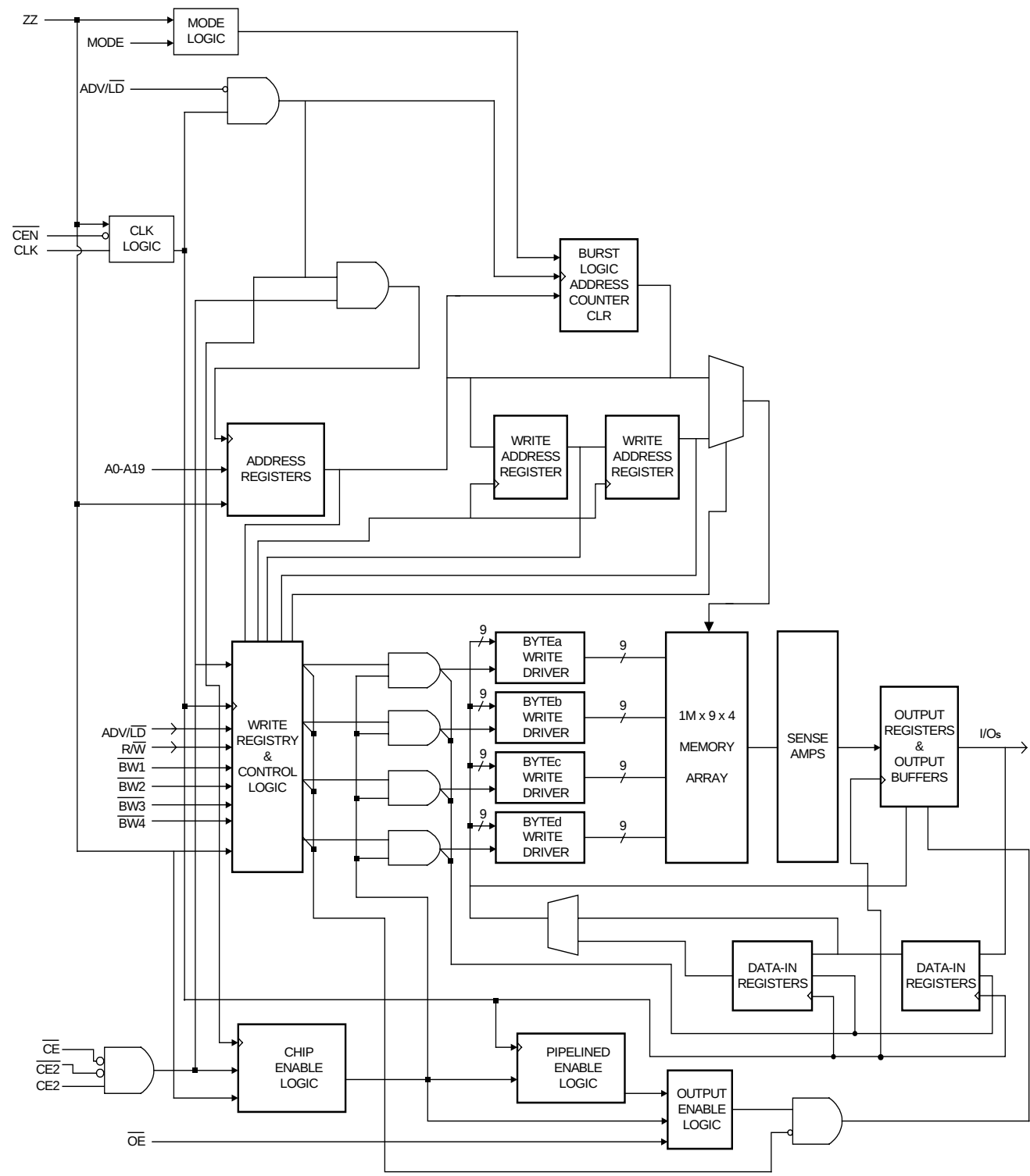
Block Diagram (1M X 36)
