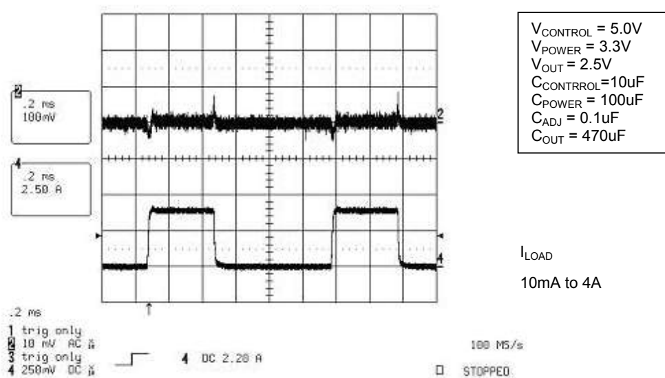
Transient Response
