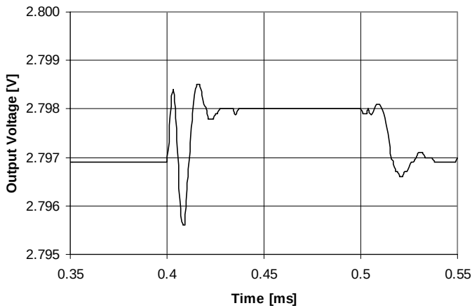
Transient Line Regulation at Full Load in Low Power Mode
