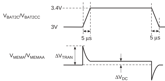
Figure 4. Line Regulation
