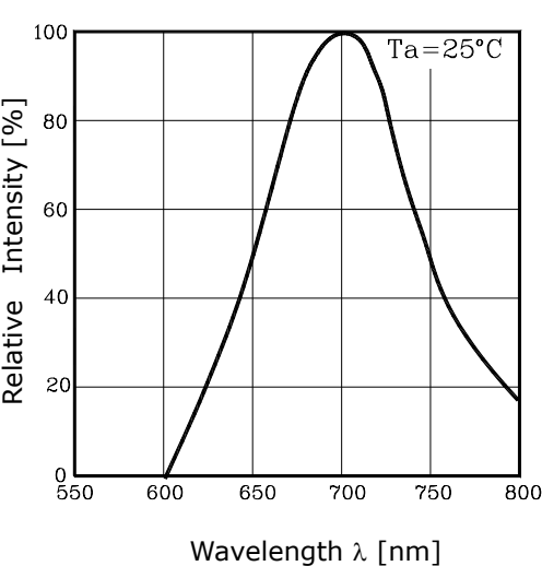
Fig. 4 Spectrum Distribution
