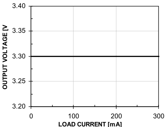
Load Regulation (VIN = 5V)
