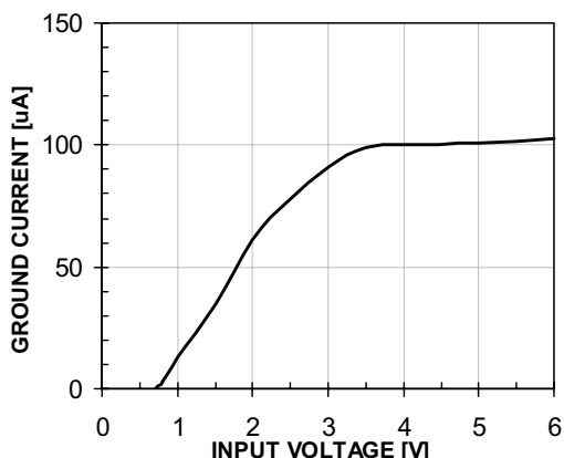
Ground Current vs. Input (5mA Load)
