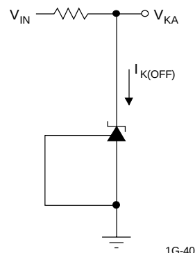
TEST CIRCUIT 3
