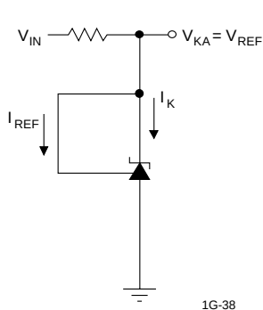
TEST CIRCUIT 1
