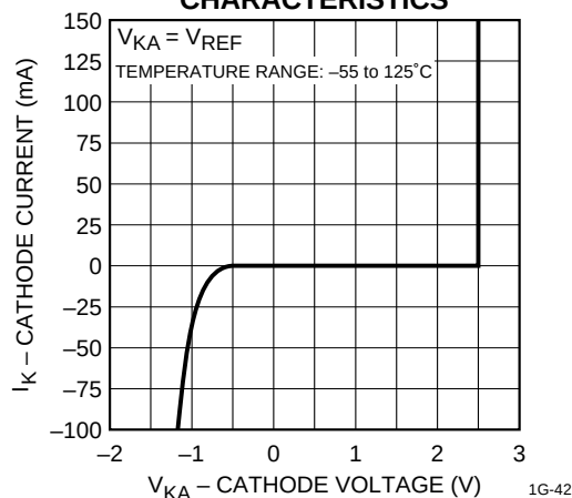
HIGH CURRENT OPERATING CHARACTERISTICS
