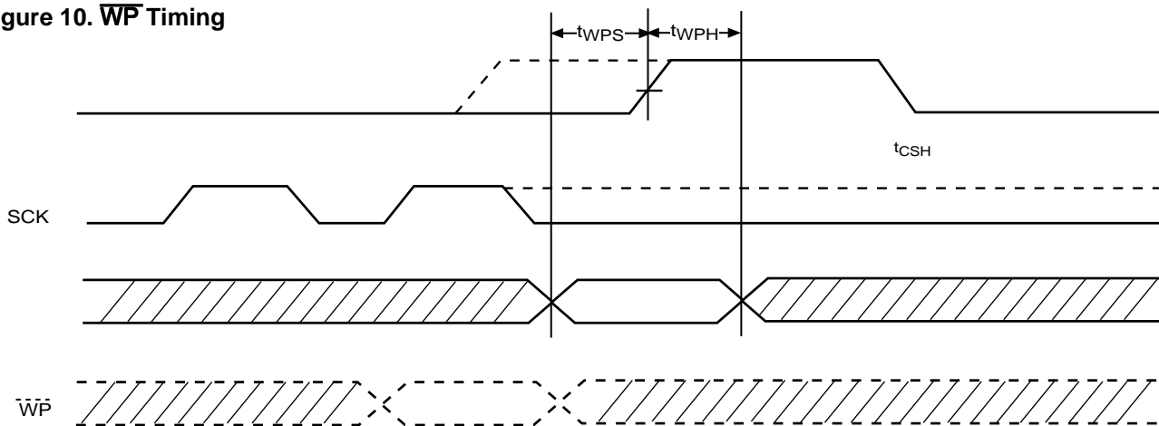
Figure 10. WP Timing
