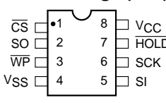
DIP Package (P, L)
