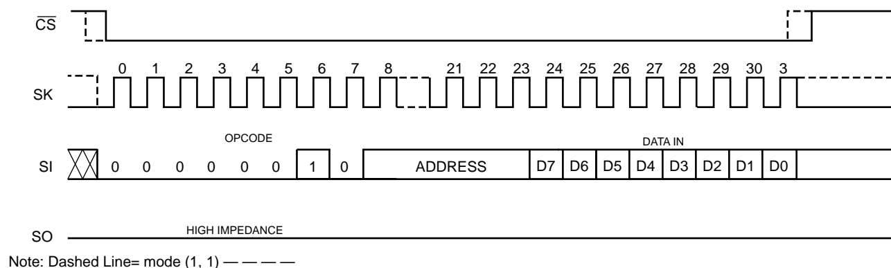
Figure 7. WRSR Timing
