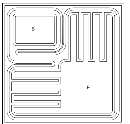
BACKSIDE COLLECTOR
