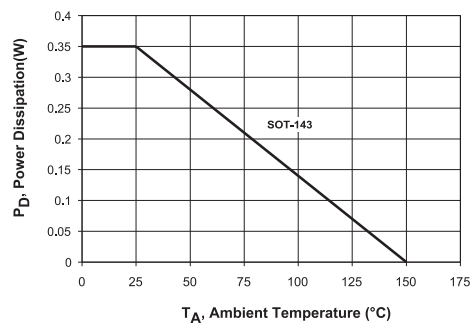
Power Derating
