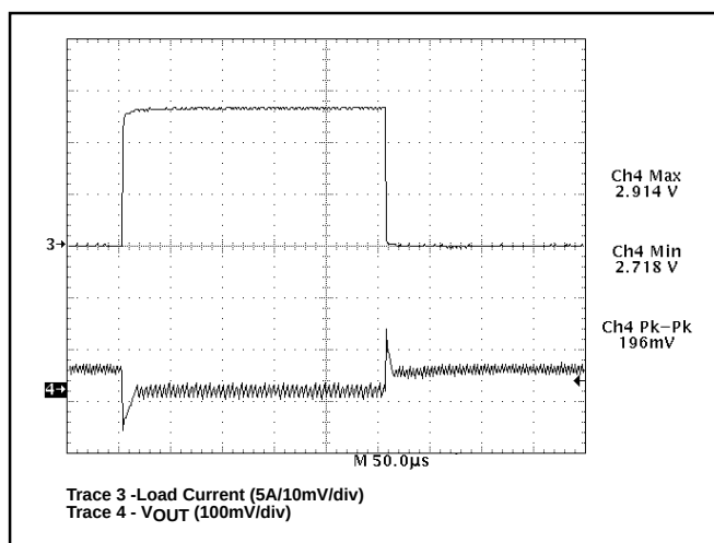
Figure 7: Output Voltage Transient Response to a 14A load pulse, V_{OUT} = +2.84V (DAC = 10111).
