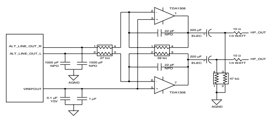
Figure 18. Stereo Output
