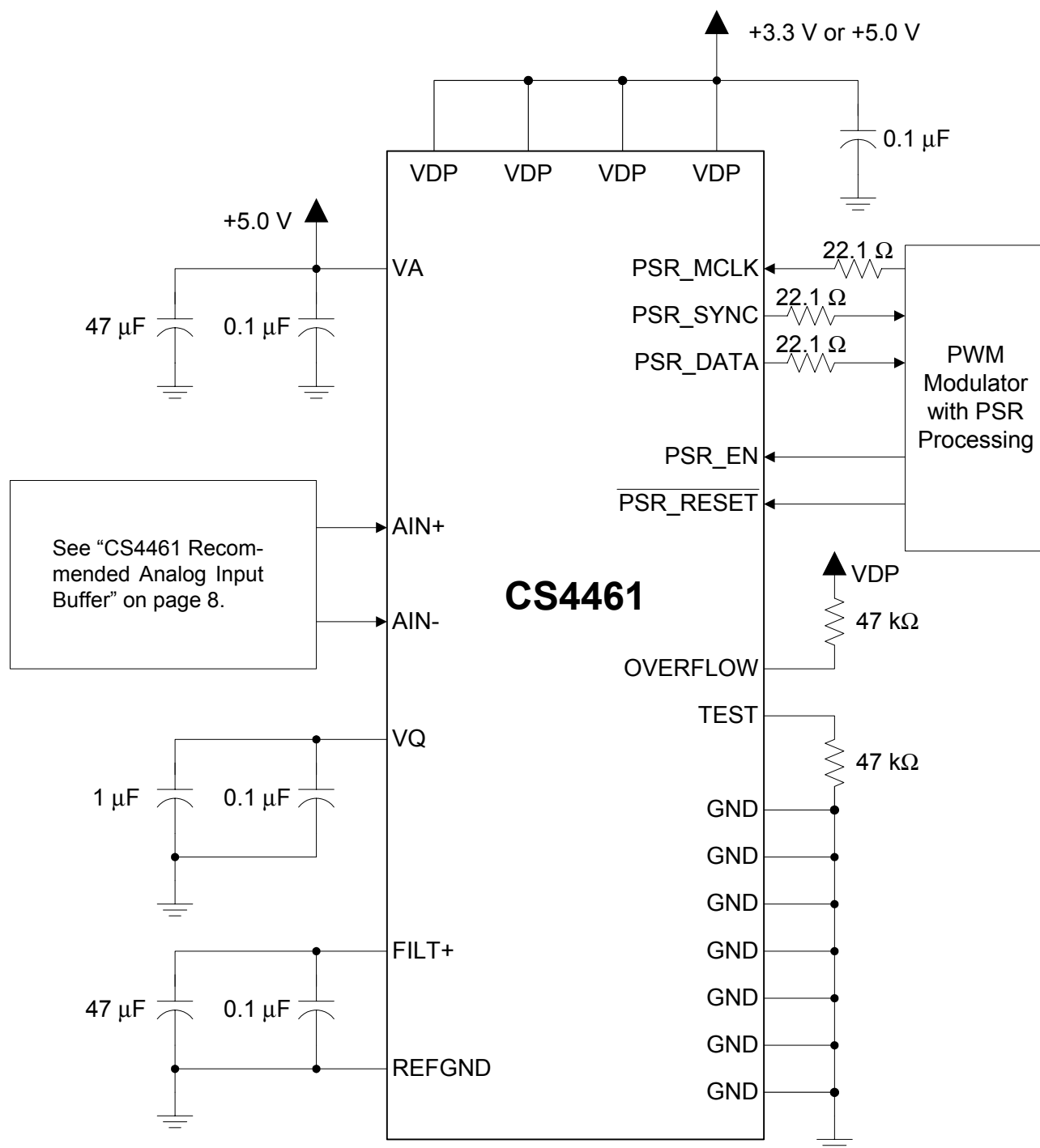
Figure 1. Typical Connection Diagram
