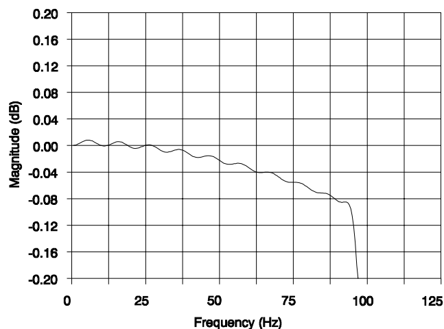
Figure 6. CS5322 Digital Filter Passband Ripple f_0 = 250 Hz
