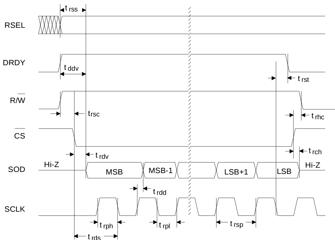
Serial Port Read Timing
