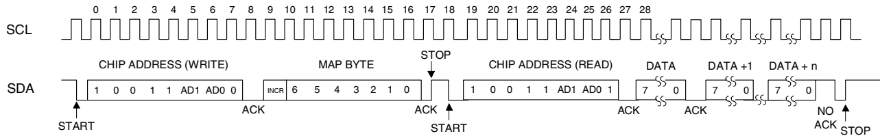
Figure 12. Control Port Timing, I²C Read
