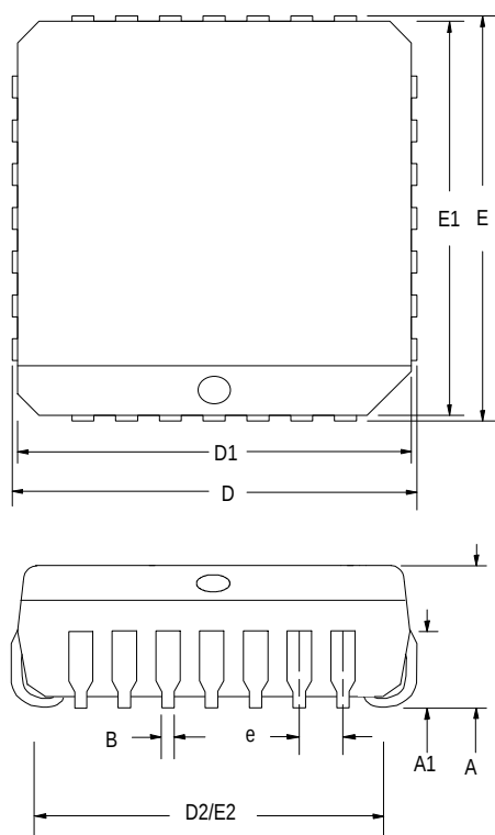
28-pin PLCC
