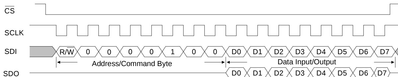
Figure 13. Input/Output Timing
