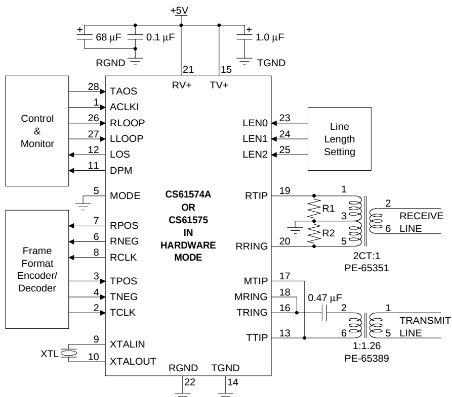
Figure A2. 120 \Omega , E1 Hardware Mode Configuration
