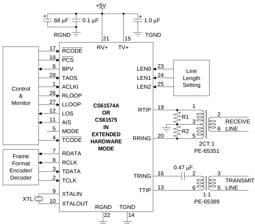
Figure A3. 75 \Omega , E1 Extended Hardware Mode Configuration
