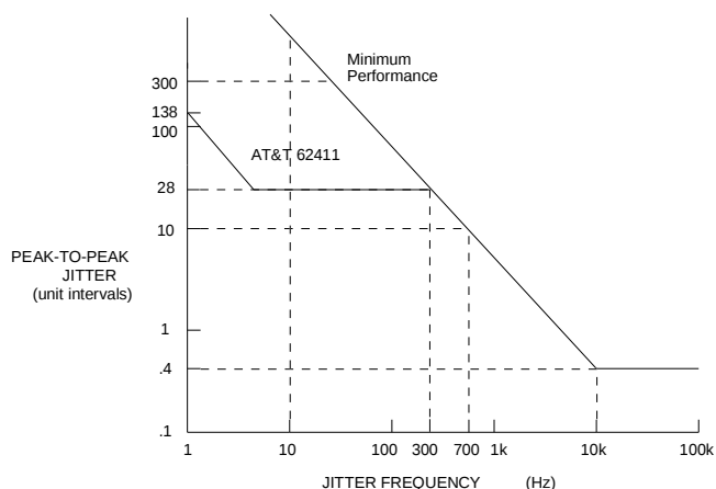
Figure 11. Minimum Input Jitter Tolerance of Receiver
