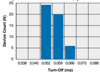
TS190L Typical Turn-Off Time (N=50 Ambient Temperature = 25°C) (Load Current = 150mADC; I F = 5mADC)
