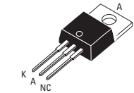
TO-220AB Non-Isolated (CRNB25...L3)
