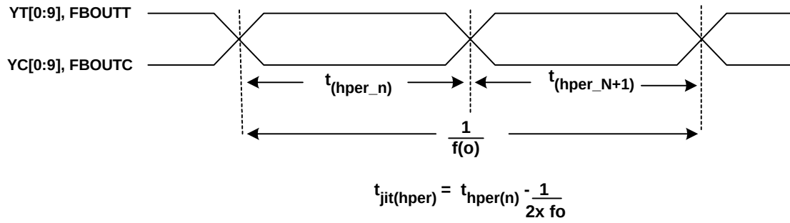
Figure 4. Half-Period Jitter
