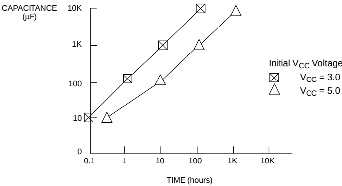
DATA RETENTION TIME VS. CAPACITANCE Figure 11
