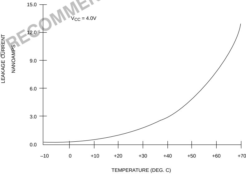
TYPICAL LEAKAGE CURRENT VS. TEMPERATURE Figure 7
