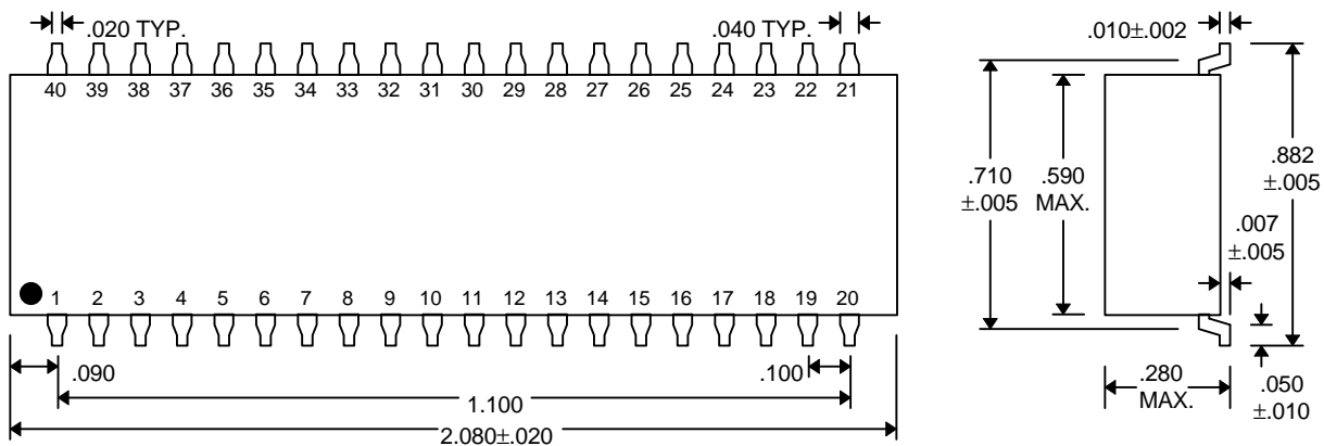
Gull-Wing (PPG38F-xxC5, PPG38F-xxMC5)
