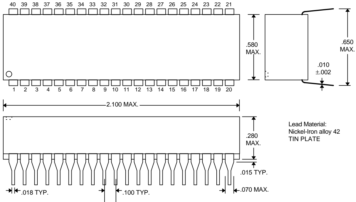
DIP (PPG38F-xx, PPG38F-xxM)
