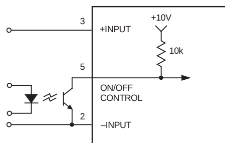
Figure 6. Driving the On/Off Control Pin
