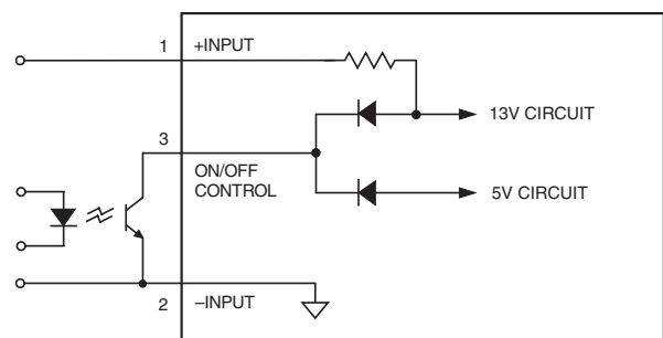
Figure 1. Internal On/Off Control circuitry
