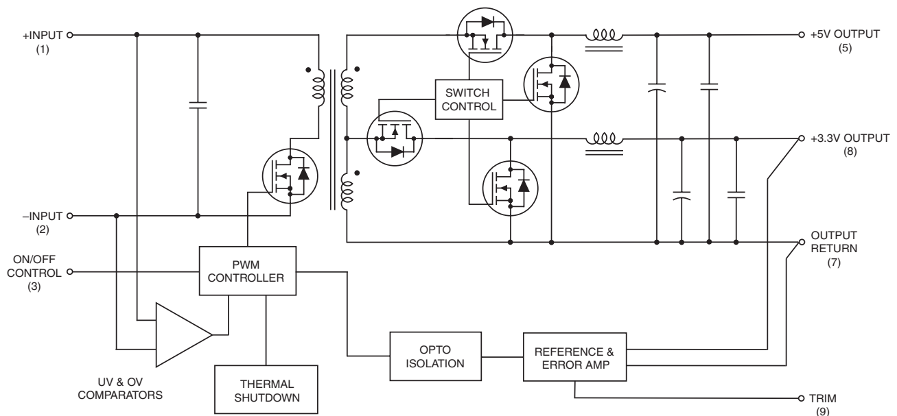
Figure 1. Simplified Schematic
