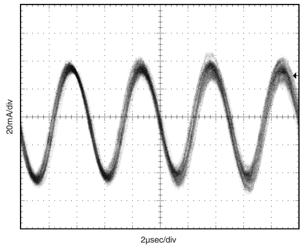
Input Reflected Ripple Current ( V_{IN} = 12V , V_{OUT} = 5V/10A , C_{IN}/C_{OUT} = 22\mu F )
