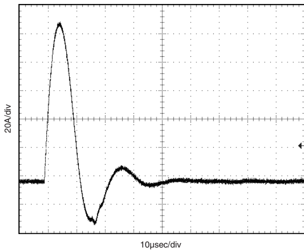
Input Inrush Current ( V_{IN} = 12V , 7000 \mu F as Input Switch)
