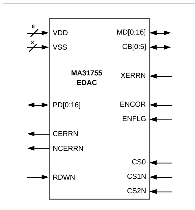
Figure 1: Chip Signals
