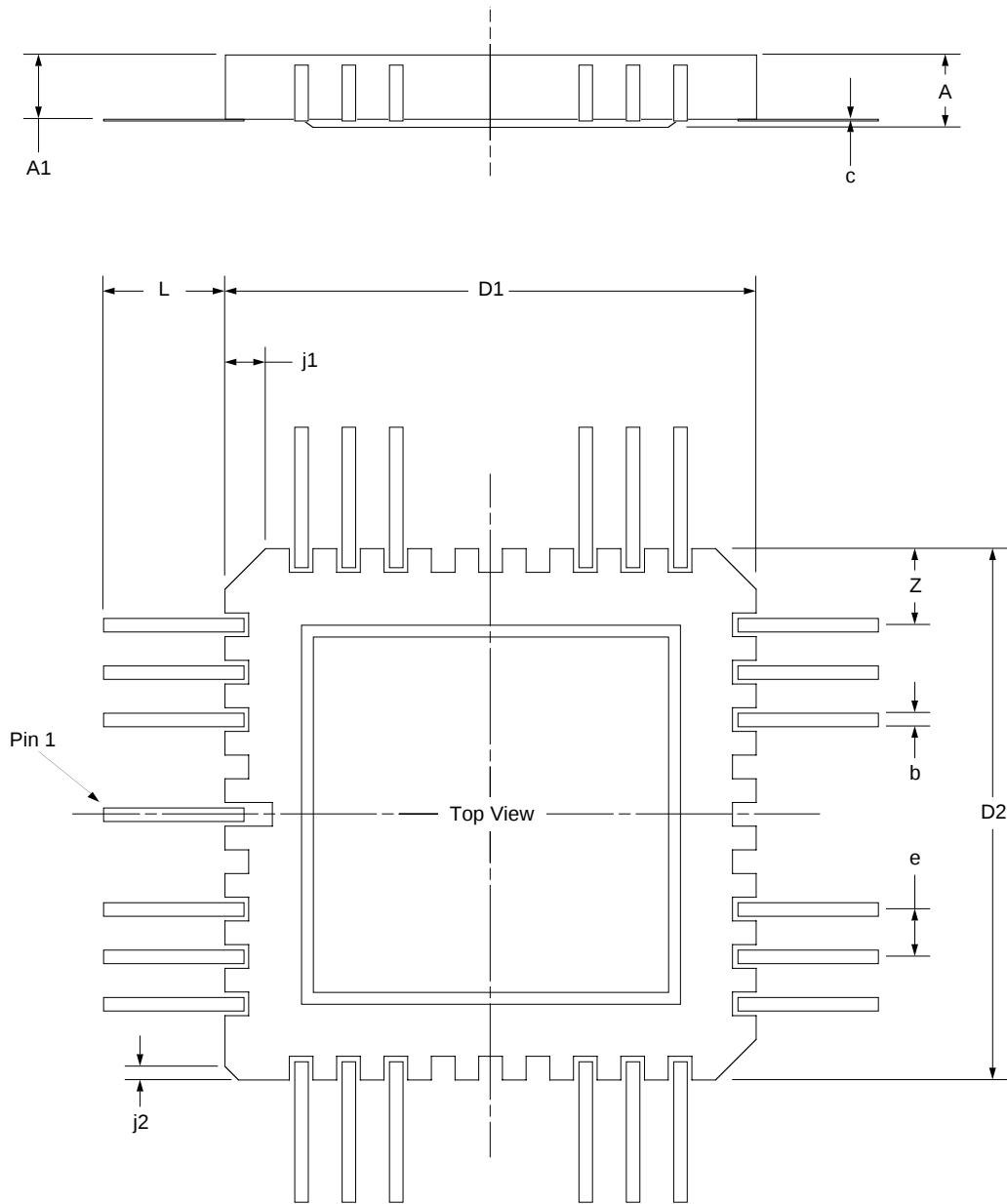
Figure 17: Dimensioned Drawing for the 68-pin Flatpack Package Topbrazed
