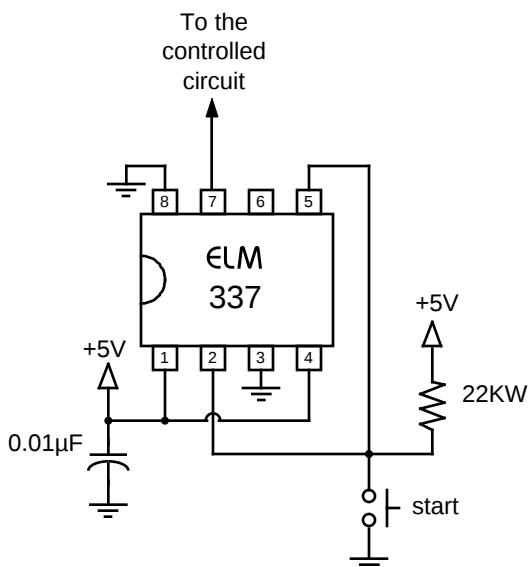
Figure 2. Time Delay Dropout Switch
