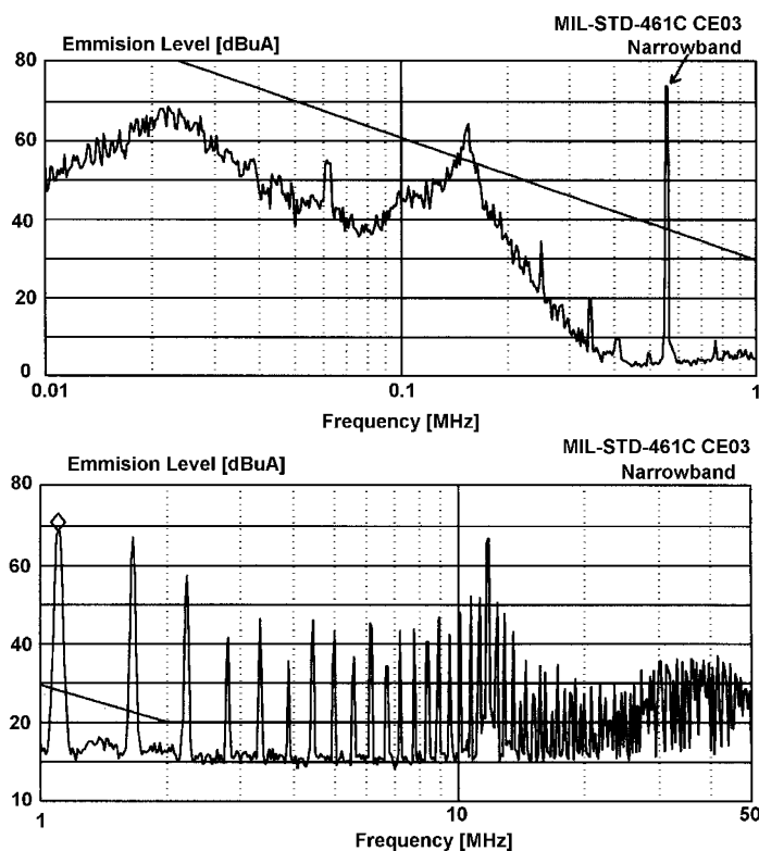
Figure 7 – MIL-STD-461C DV200-2815D Without EMI Filter
