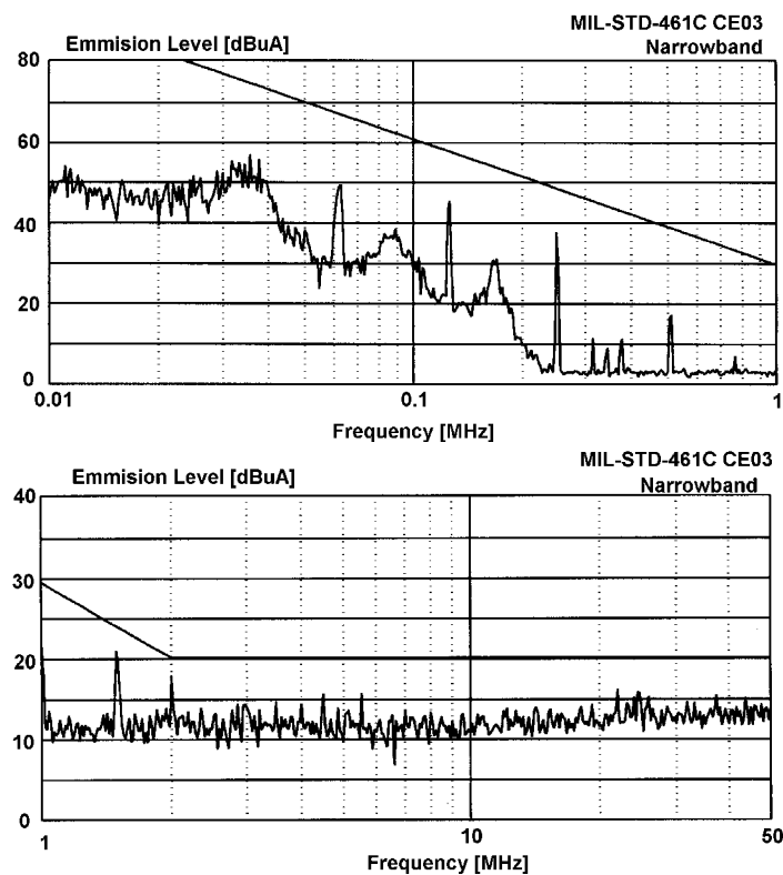
Figure 8 – MIL-STD-461C DV200-2805S With DVMN28 EMI Filter
