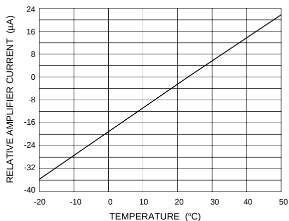
Fig. 10 Amplifier Current vs Temperature
