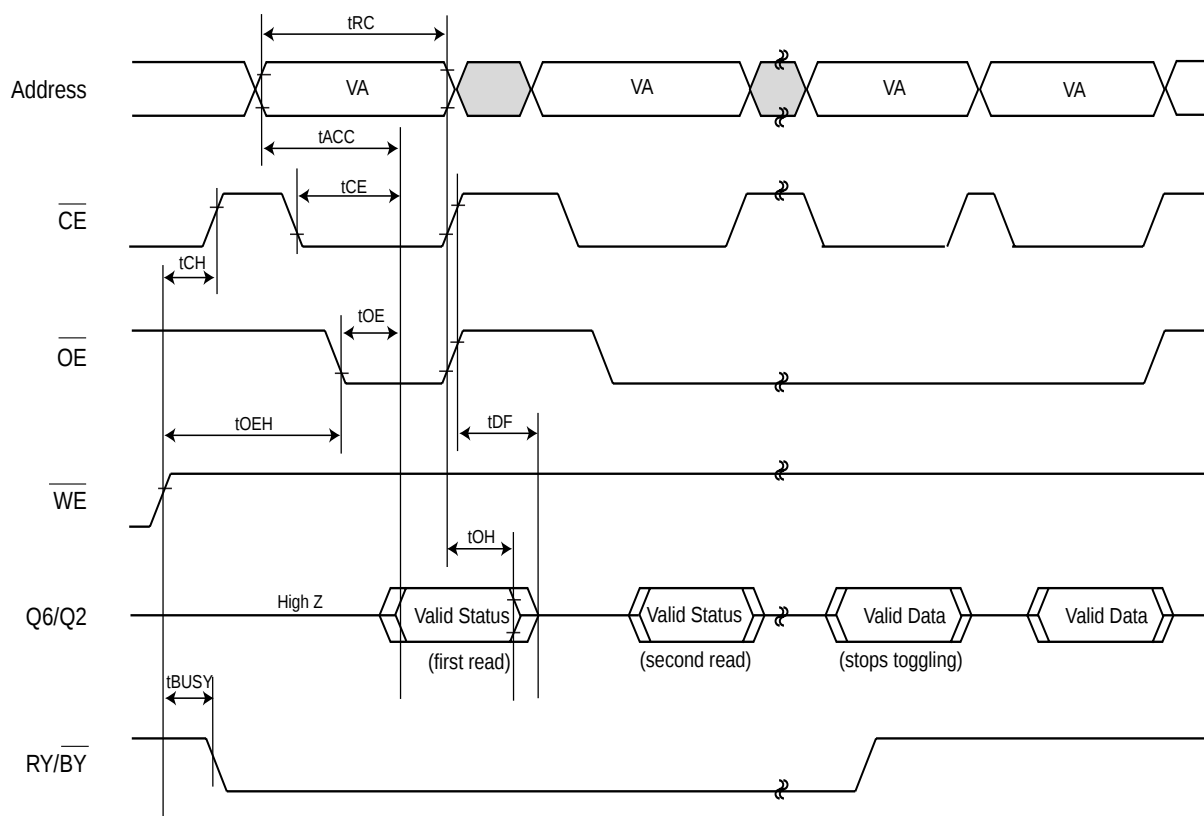
Figure 21. TOGGLE BIT TIMING WAVEFORMS (DURING AUTOMATIC ALGORITHMS)
