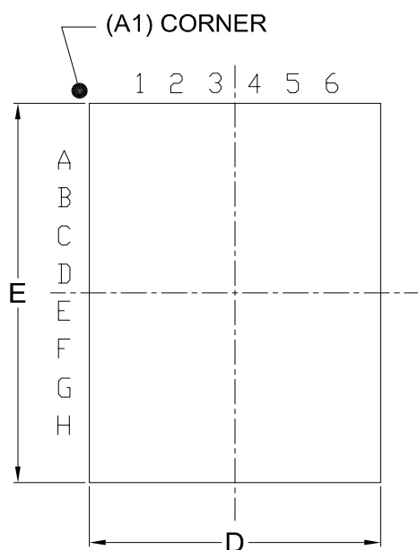
TOP VIEW
