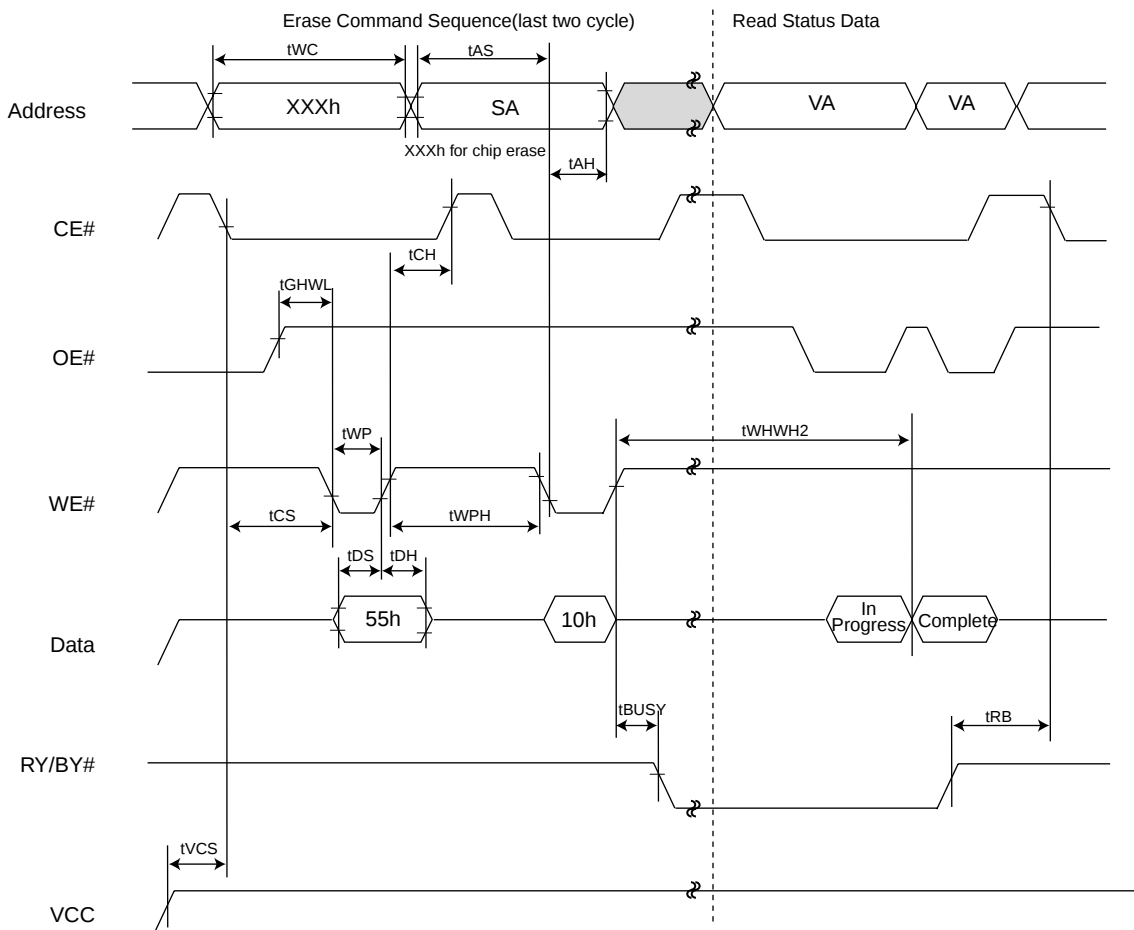
Figure 4. AUTOMATIC CHIP ERASE TIMING WAVEFORM
